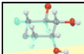
Fig. 3. Chair conformation of the six-membered ring.
