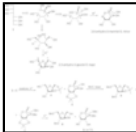
Fig. 1. Two possibilities of dehydration of D -mannitol relevant to the synthesis of 1,5-anhydro- D -mannitol and formation of the dibenzyl ethers.
