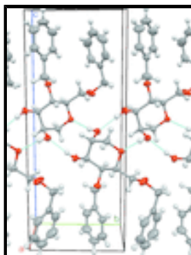
Fig. 4. Infinite chain of 2,6-anhydro-1,3-di- O -benzyl- D -mannitol molecules along the b axis. View along the a axis.
