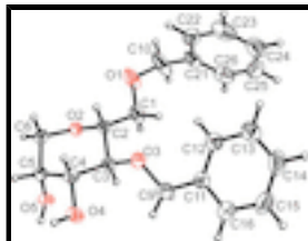
Fig. 2. ORTEP view of 1,5-anhydro-4,6-di- O -benzyl- D -mannitol with displacement ellipsoids drawn at the 50% probability level.
